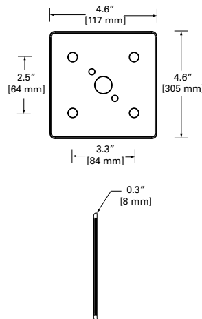
Mounting Plate
