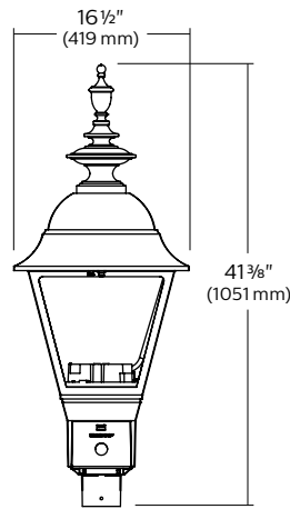
VX152 Height: 41-3/8" (105 cm) Width: 16-1/2" (42 cm) Max EPA: 1.65 sq. ft. Max Weight: 27.9 lbs (12.7 kg)
