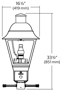
VX151 Height: 33-1/2" (85 cm) Width: 16-1/2" (42 cm) Max EPA: 1.65 sq. ft. Max Weight: 27.9 lbs (12.7 kg)
