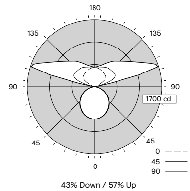
Definition Symmetric Flush Silk Lens – LQ Spacing Criteria: 1.23/1.21
