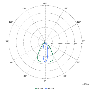
Polar Normal (separate) - ST770T1 - 910505101382
