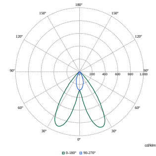
Polar Normal (separate) – ST760TI – 910505102530
