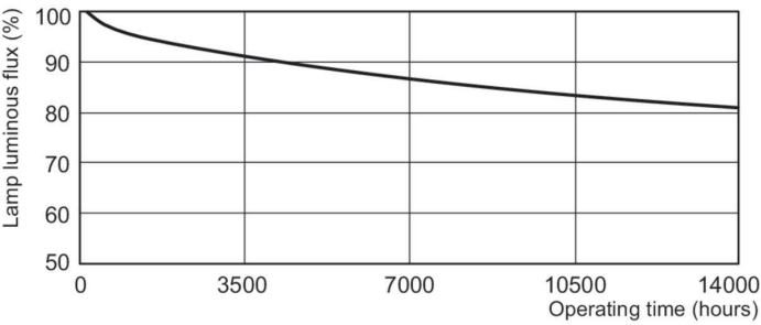
Lumen Maintenance Diagram - PL-S 13W/850/2P 1CT/5X10BOX ALTO
