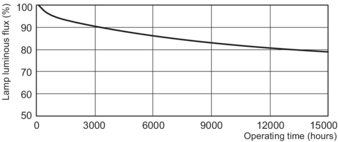
Lumen Maintenance Diagram - MASTER PL-C 26W/840/4P 1CT/5X10BOX
