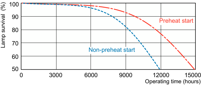
Life Expectancy Diagram - MASTER PL-C 26W/840/4P 1CT/5X10BOX
