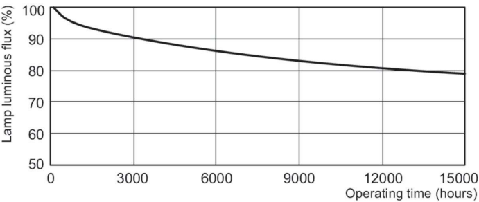
Lumen Maintenance Diagram - PL-C 26W/41/4P/ALTO 10PK
