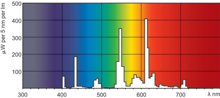
Spectral Power Distribution Colour - PL-T 42W/830/A/4P 1CT/5X10BOX ALTO
