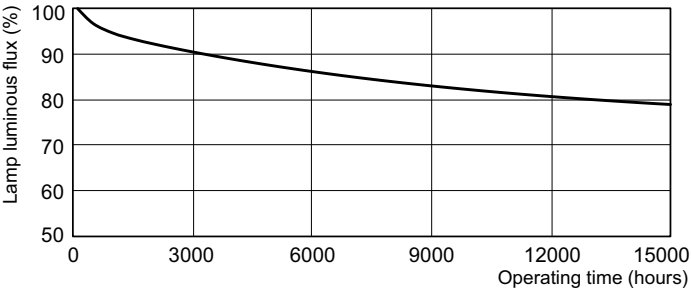
Lumen Maintenance Diagram - PL-T 42W/830/A/4P 1CT/5X10BOX ALTO
