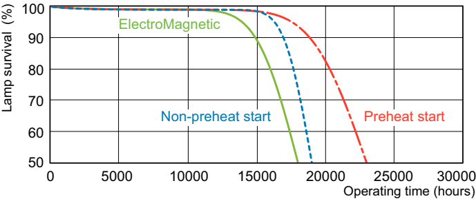
Life Expectancy Diagram - TL-D 18W/827 1SL/25
