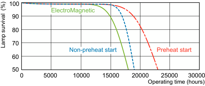
Life Expectancy Diagram - TL-D 30W/840 1SL/25
