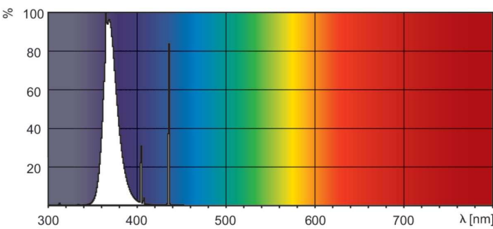
Spectral Power Distribution Colour - Actinic BL TL-D 18W/10 Secura 1SL/25
