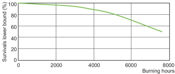
LDLE_MHN-FC_2200W_640-Life expectancy diagram
