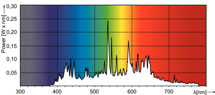
Spectral Power Distribution Colour - MASTERC CDM-TC Elite 50W/942 G8.5 1CT
