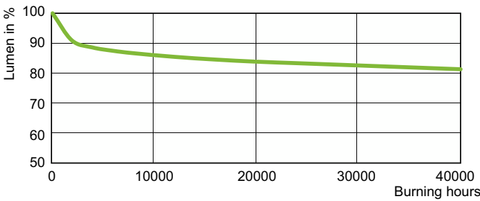
Lumen Maintenance Diagram - MST SON APIA Plus Xtra 70W E27 1SL/24
