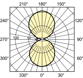
Light Distribution Diagram - MST SON-T PIA Plus 100W/220 E40 1SL/12
