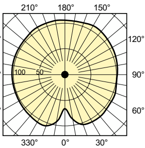
Light Distribution Diagram - MST SON-T PIA Plus 100W/220 E40 1SL/12
