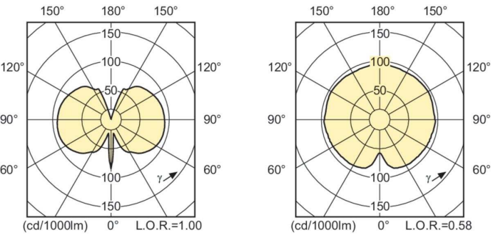
Light Distribution Diagram - CDM20/TC/830 Elite
