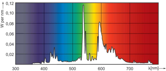
Spectral Power Distribution Colour - CDM20/TC/830 Elite
