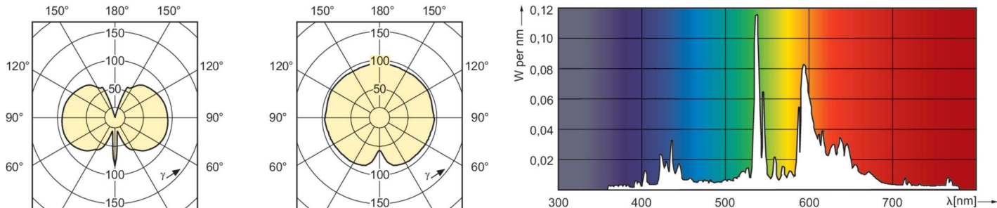
Light Distribution Diagram - MASTERC CDM-TC Elite 20W/830 G8.5 1CT/12
