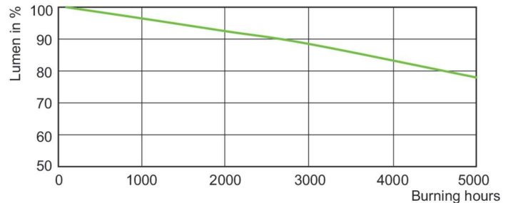
Lumen Maintenance Diagram - MASTER MHN-SA 2000W/956 400V XW HO UNP/1
