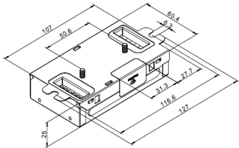
Enclosure XI036C100V054DSM1 (bottom entry)
