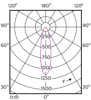
Light Distribution Diagram - MAS LED ExpertColor 5.5-50W GU10 930 25D
