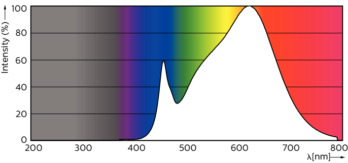
Spectral Power Distribution Colour - MAS LEDspotVLE D 4.9-50W GU10 930 36D UK
