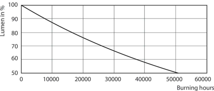
Lumen Maintenance Diagram - MAS LEDspotVLE D 4.9-50W GU10 930 36D UK
