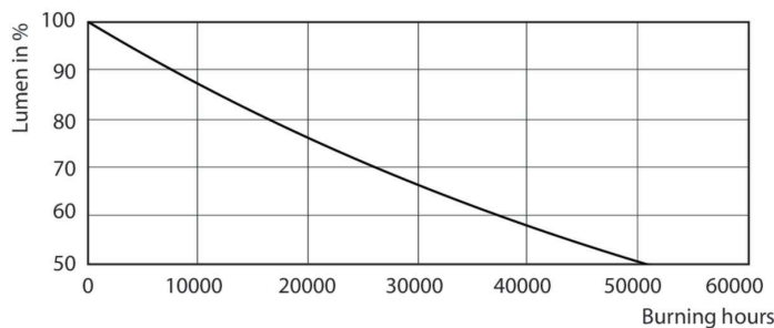
Lumen Maintenance Diagram - MAS LED spot VLE D 4.9-50W GU10 940 60D
