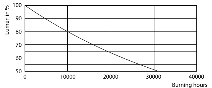
Lumen Maintenance Diagram - CorePro LEDBulbND 7-60W E27 WW A60 CL
