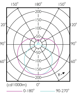
Light Distribution Diagram - 8T5HE/22-835/IF10/G/DIM 10/1
