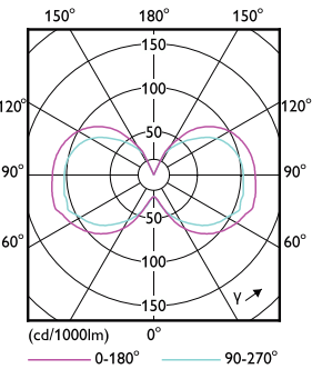
Light Distribution Diagram - 3.6T3/PER/830/ND/G9/120V 6/3PF
