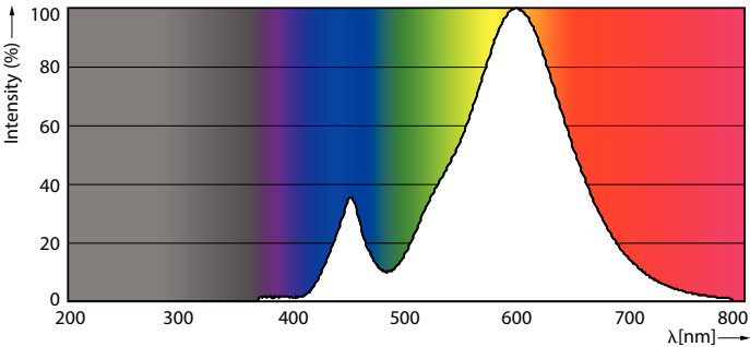
Spectral Power Distribution Colour - ESS LEDspot 5W 400lm GU5.3 827 220V
