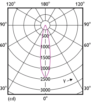
Light Distribution Diagram - MASTER LED 6.5-50W 930 MR16 24D CN
