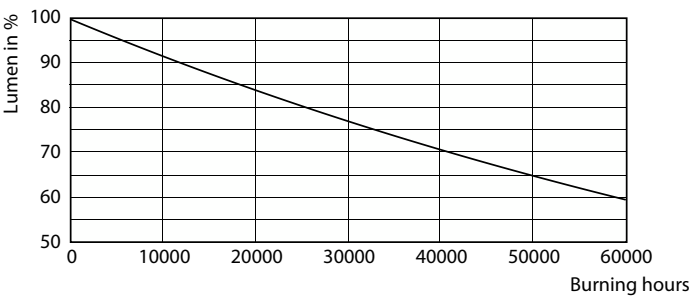
Lumen Maintenance Diagram - MASTER LED 6.5-50W 930 MR16 24D CN
