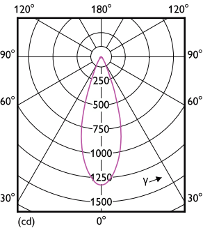
Light Distribution Diagram - MASTER LED 6.5-50W 927 MR16 36D CN
