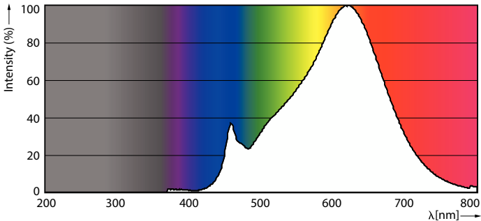
Spectral Power Distribution Colour - MASTER LED 6.5-50W 927 MR16 36D CN
