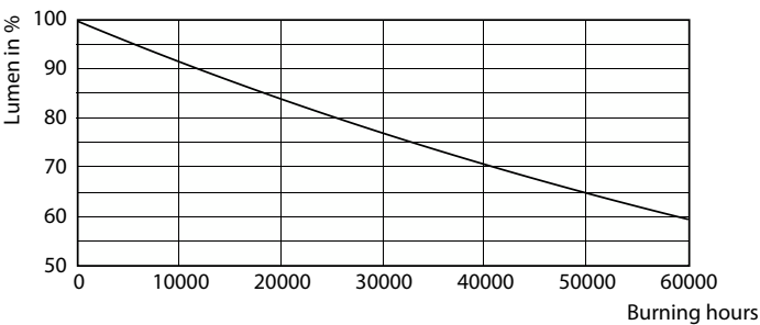
Lumen Maintenance Diagram - MASTER LED 6.5-50W 930 MR16 36D CN
