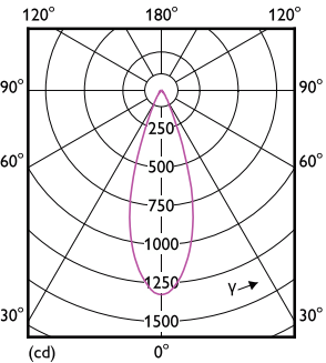
Light Distribution Diagram - MASTER LED 6.5-50W 930 MR16 36D CN
