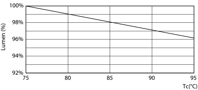
Lumen Maintenance Diagram - 5.5PL-C/LED/13H/830/IF5/P/4P 20/1
