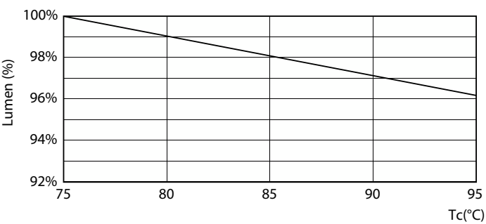
Lumen Maintenance Diagram - 5.5PL-C/LED/13H/835/IF5/P/4P 20/1
