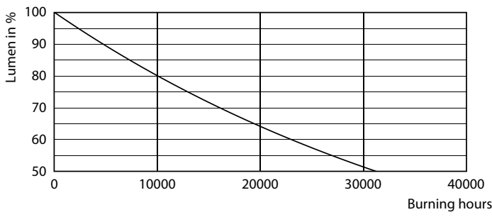
Lumen Maintenance Diagram - CorePro LEDLusterND4.3-40W E27 827P45CLG
