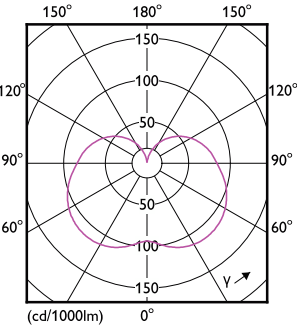
Light Distribution Diagram - LEDStick 9.5W B22 3000K 1PF/6 AU
