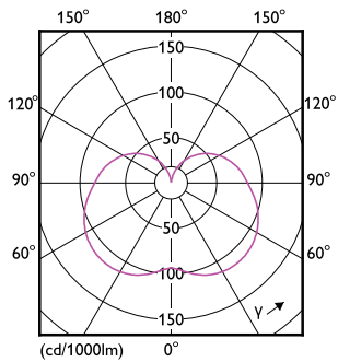
Light Distribution Diagram - LEDStick 9.5W B22 6500K 1PF/6 AU
