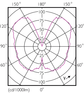
Light Distribution Diagram - 7.5T20/VIN/820/CL/G/E26/amber/SP/DIM 1CT
