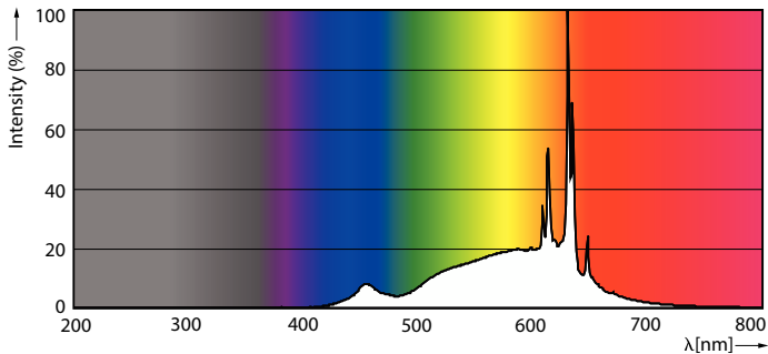
Spectral Power Distribution Colour - 5A19/MAS/927-22/FR/P/E26/T20 6/1CT
