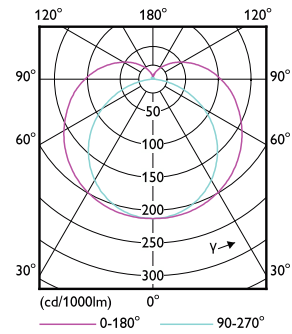
Light Distribution Diagram - 8.5T8/MAS/36-850/IF14/P/DIM 10/1
