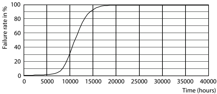
Life Expectancy Diagram - 8A19/LED/YELLOW/P/ND 120V 4/1FB
