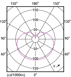
Light Distribution Diagram - 8A19/LED/YELLOW/P/ND 120V 4/1FB
