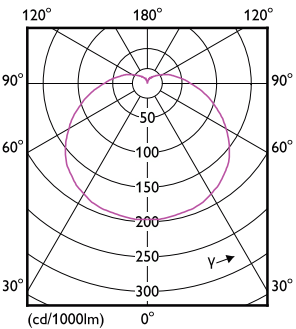
Light Distribution Diagram - 8A19/LED/PURPLE/ND 120V 4/1FB
