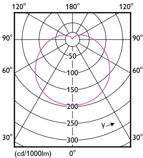
Light Distribution Diagram - LEDBulb 14.5W B22 6500K 230VA67 1CT/6APR
