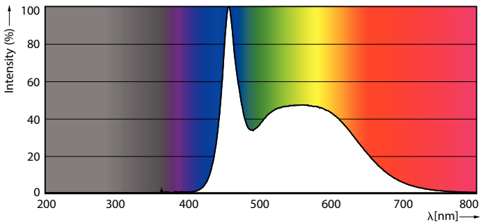
Spectral Power Distribution Colour - LEDBulb 14.5W B22 6500K 230VA67 1CT/6APR
