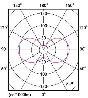
Light Distribution Diagram - CorePro LEDLusterND6.5-60W P45 E27840FRG
