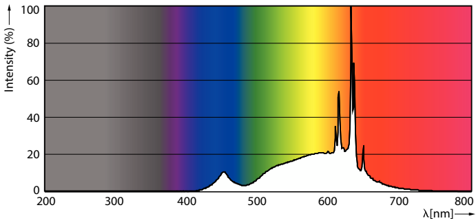
Spectral Power Distribution Colour - 5A19/COR/927/FR/P/E26/DIM/T20 6/1CT
