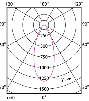
Light Distribution Diagram - 9.4PAR30S/COR/930/F40/DIM/120V T20 6/1FB
