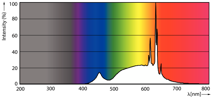
Spectral Power Distribution Colour - 9.4PAR30S/COR/930/F40/DIM/120V T20 6/1FB
