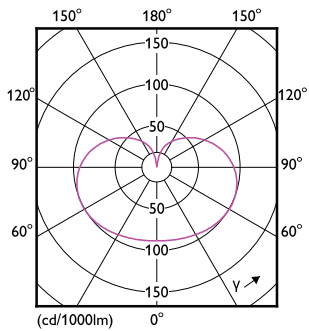
Light Distribution Diagram - LED Sensor 8-60W E27 CDL FR 1PF/6 APR
