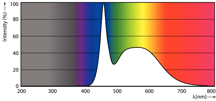
Spectral Power Distribution Colour - LED Sensor 8-60W E27 CDL FR 1PF/6 APR
