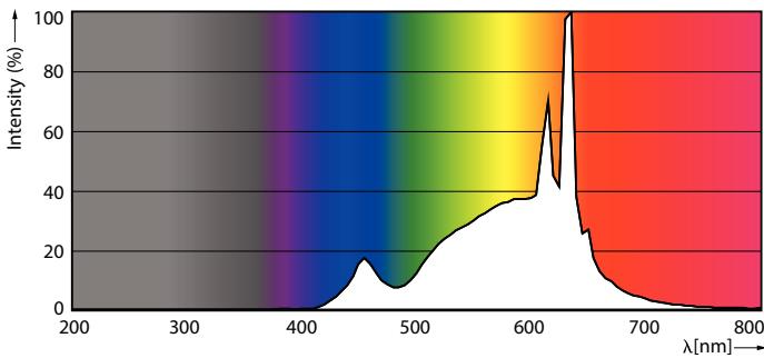
Spectral Power Distribution Colour - LEDBulb 10.5-75W B22 2700K D 1PF/6 AU
