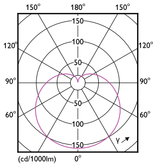
Light Distribution Diagram - LEDBulb 10.5-75W B22 2700K D 1PF/6 AU
