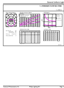
General uniform lighting - LEDBulb 10.5-75W B22 2700K D 1PF/6 AU
