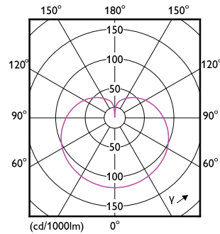
Light Distribution Diagram - 18.5A21/LED/927/P/E26/3WAY ND 4/1FB T20
