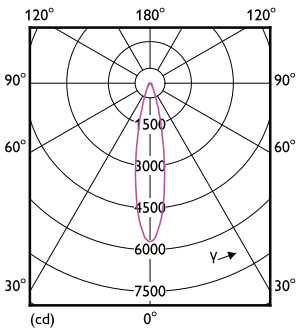
Light Distribution Diagram - LED 14-120W PAR38 827 25D
