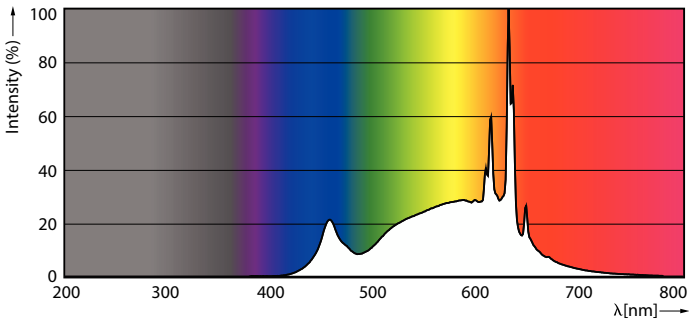
Spectral Power Distribution Colour - 12.2A19/COR/930/FR/P/E26/DIM/T20 6/1CT
