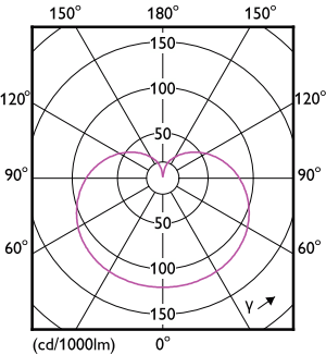
Light Distribution Diagram - 12.2A19/COR/930/FR/P/E26/DIM/T20 6/1CT
